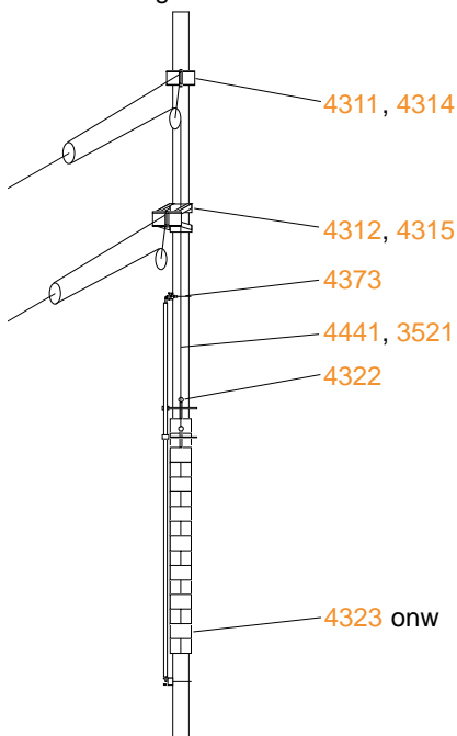
1 contact wire and 1 carrying cable counterweight tensioned
