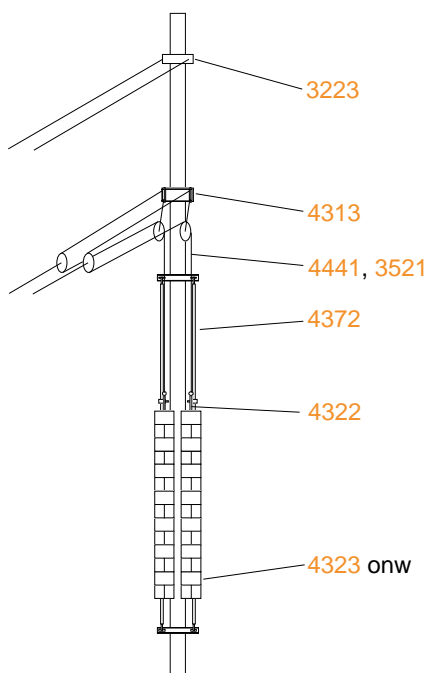
2 contact wires counterweight tensioned
