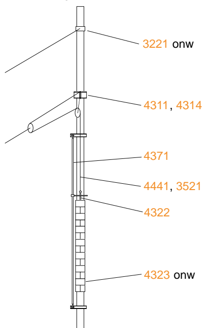
Counterweight tensioned contact wire
