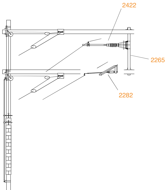
Counterweight tensioned contact wire and carrying cable
