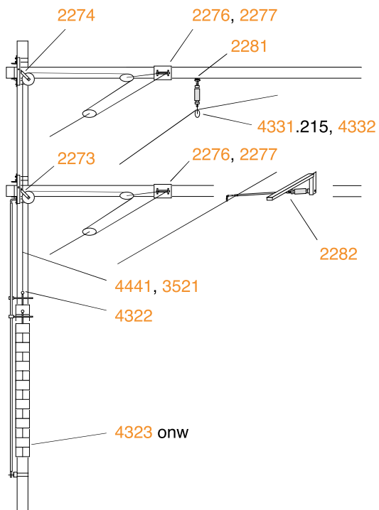
Counterweight tensioned contact wire and carrying cable
