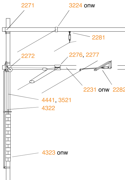
Counterweight tensioned contact wire, fixed termination for carrying cable
