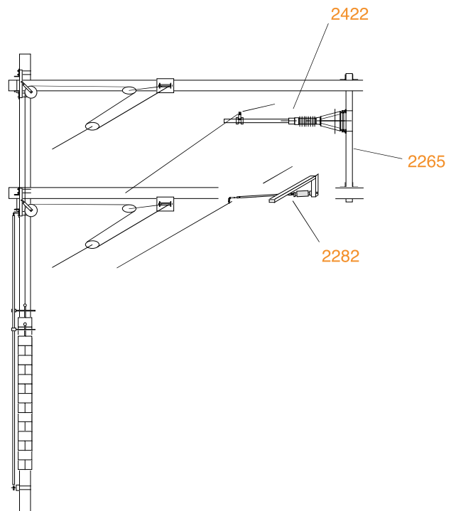
Counterweight tensioned contact wire and carrying cable
