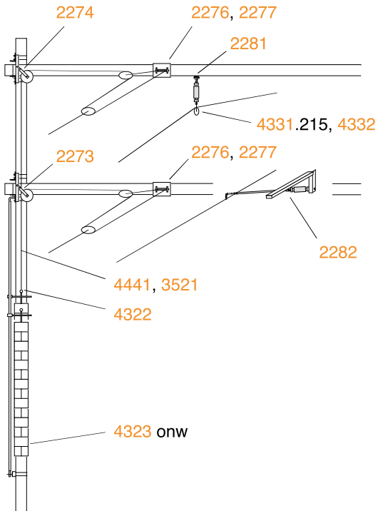
Counterweight tensioned contact wire and carrying cable
