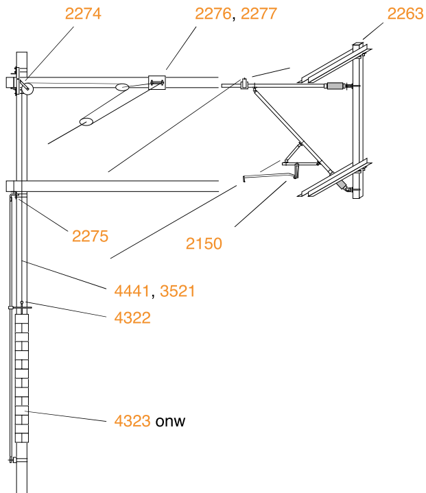
Counterweight tensioned carrying cable
